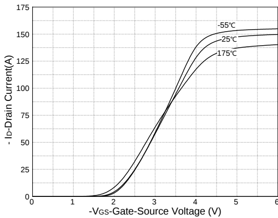
Figure 11: Transfer Characteristics
