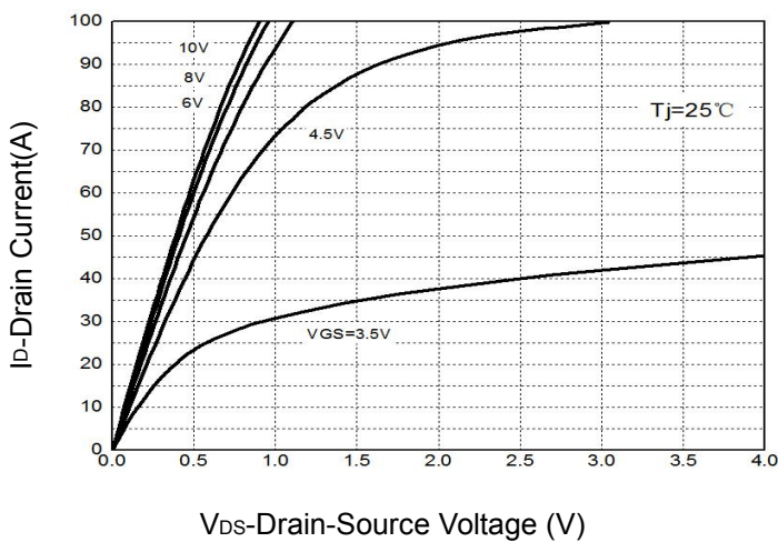
Figure 5: Output Characteristics
