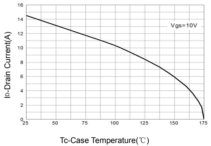
Figure 2: Drain Current
