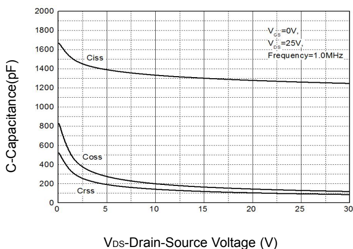
Figure 11: Capacitance Characteristics
