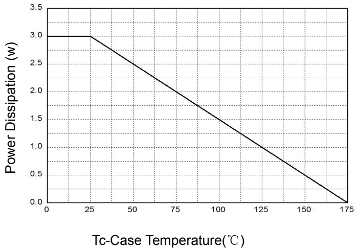
Figure 1: Power Dissipation
