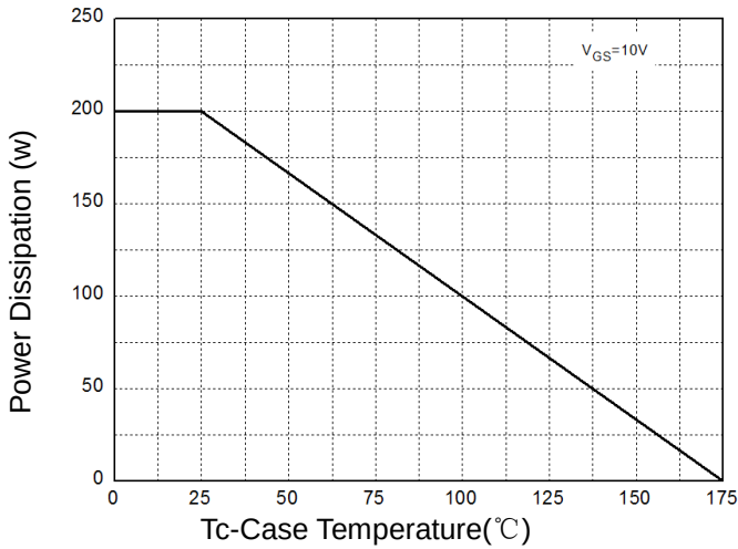
Figure 1: Power Dissipation
