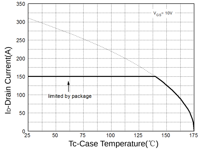
Figure 2: Drain Current
