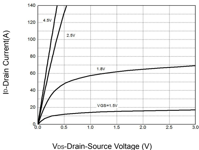
Figure 5: Output Characteristics
