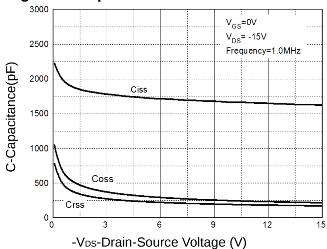
Figure 9: Capacitance Characteristics
