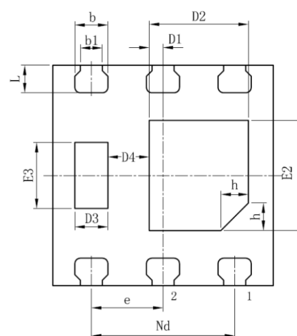
BOTTOM VIEW
