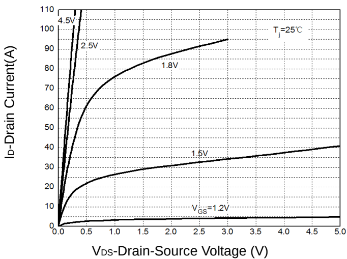
Figure 5: Output Characteristics
