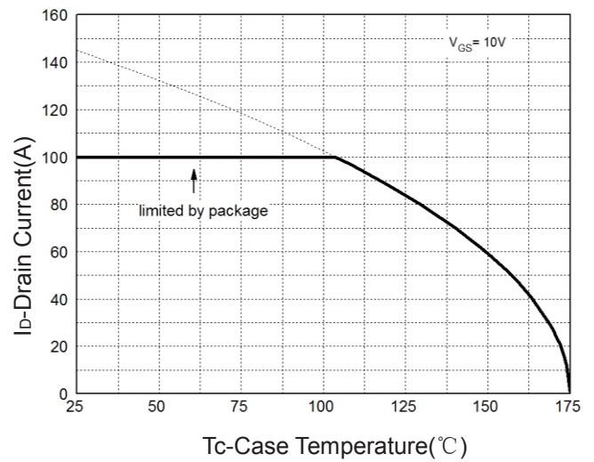
Figure 2: Drain Current
