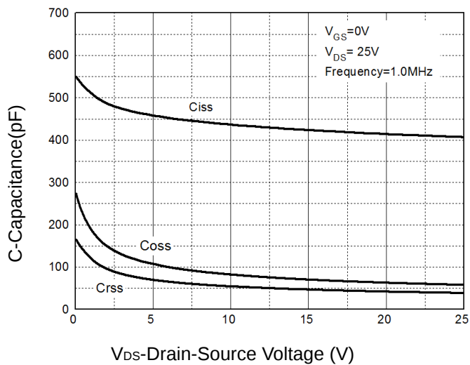
Figure 9: Capacitance Characteristics
