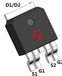
TO-252-4L
