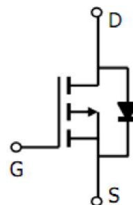
Single P-Channel MOSFET
