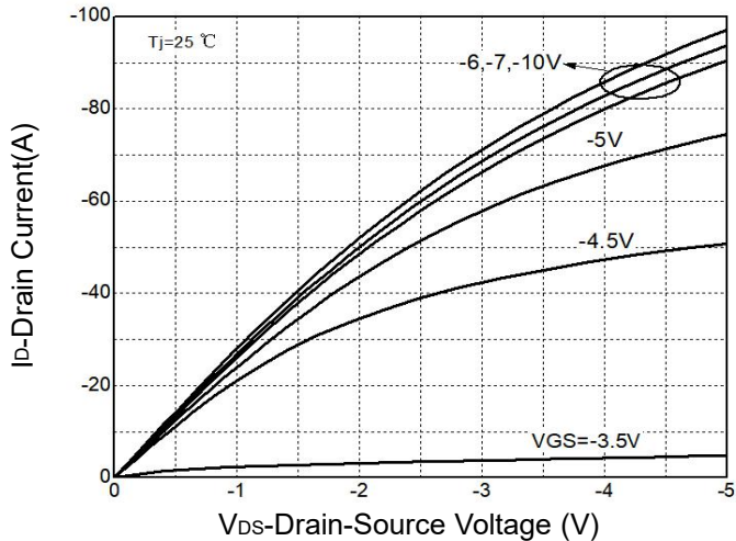
Figure 5: Output Characteristics
