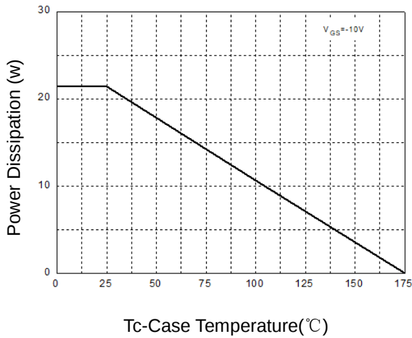
Figure 1: Power Dissipation
