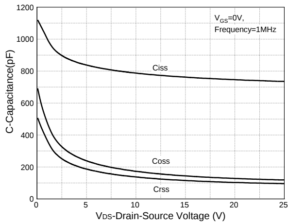
Figure 9: Capacitance Characteristics
