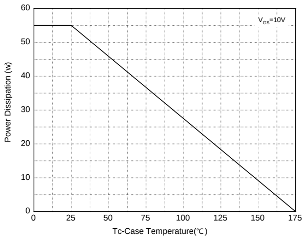
Figure 1: Power Dissipation
