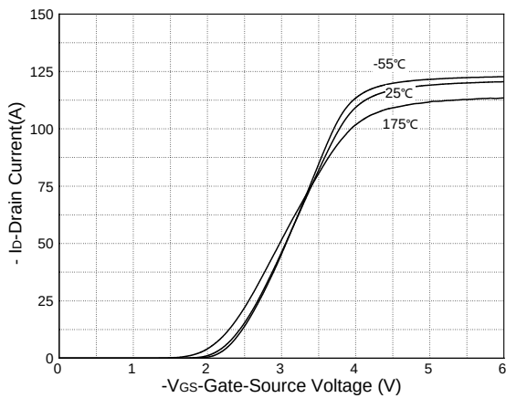
Figure 11: Transfer Characteristics
