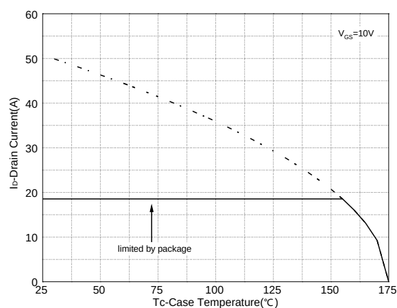
Figure 2: Drain Current
