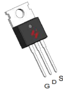
TO-220FB-3L
