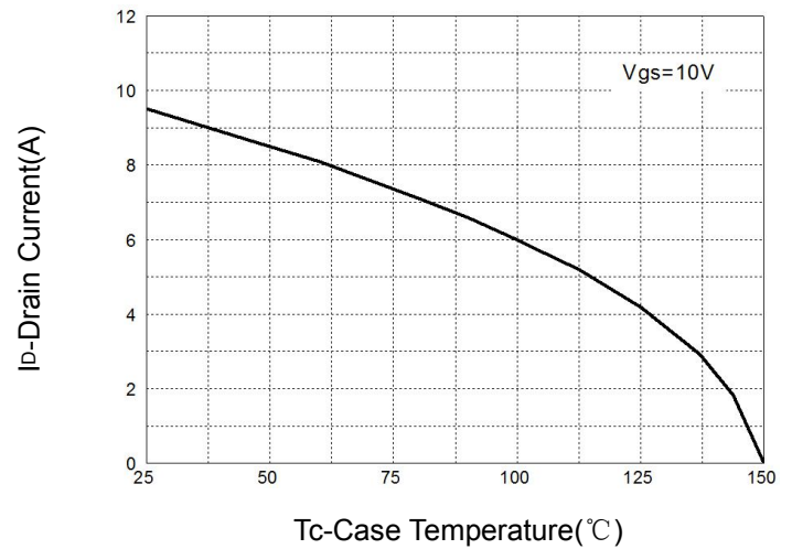
Figure 2: Drain Current
