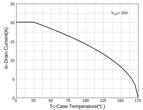
Figure 2: Drain Current
