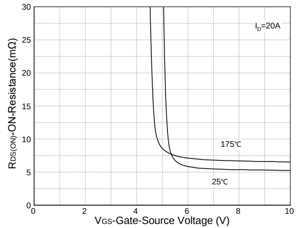
Figure 14: R_{dson} vs. Gate Voltage
