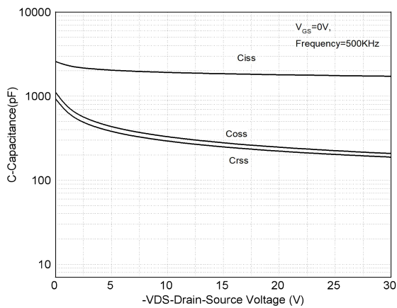
Figure 9: Capacitance Characteristics
