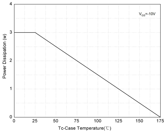
Figure 1: Power Dissipation
