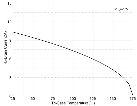
Figure 2: Drain Current
