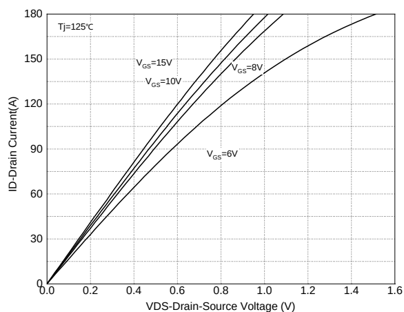
Figure 15: Output Characteristics ( 125^\circ\text{C} )
