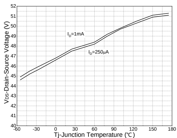
Figure 13: Drain-Source Breakdown
