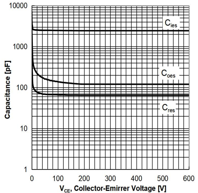
Figure 18: Typical Capacitance vs. Collector-Emirrer Voltage
