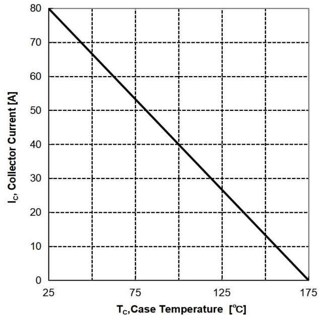
Figure 2: Collector Current vs. Case Temperature
