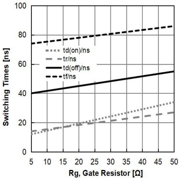
Figure 15: Typical Switching Times vs. Gate Resistor (T J =25°C, V CE =400V, V GE =15/0V, I C =15A)
