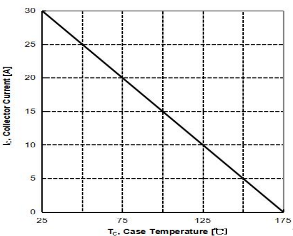
Figure 6: Collector Current vs. Case Temperature(TO-220F-3L)
