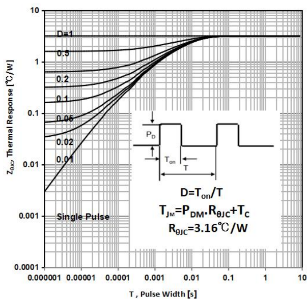
Figure 30: Diode Transient Thermal Impedance vs. Pulse Width(TO-220F-3L)
