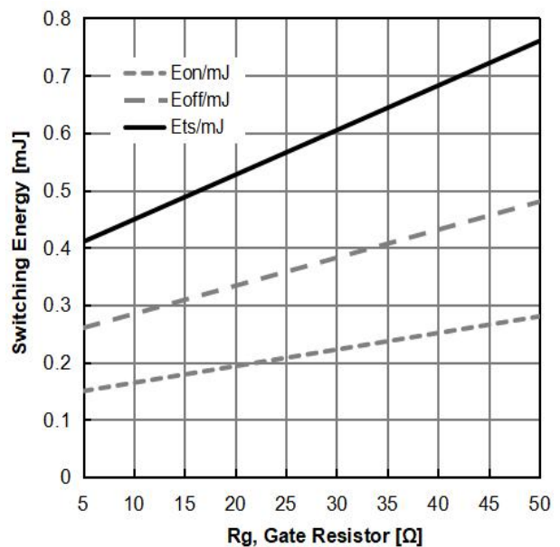
Figure 16: Typical Switching Energy vs. Gate Resistor (T J =25°C, V CE =400V, V GE =15/0V, I C =15A)
