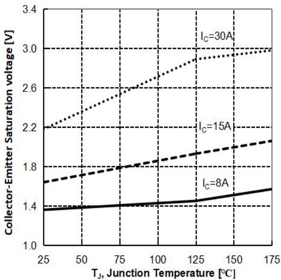
Figure 13: Typical Collector-Emitter Saturation Voltage vs. Junction Temperature
