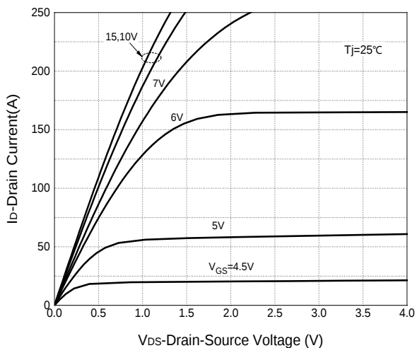
Figure 5: Output Characteristics
