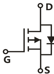
Single P-Channel MOSFET
