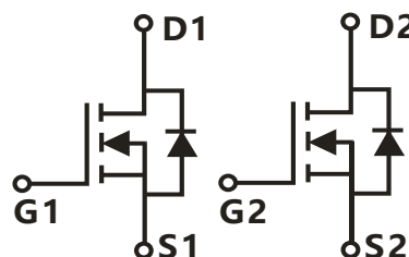
Dual N-Channel MOSFET
