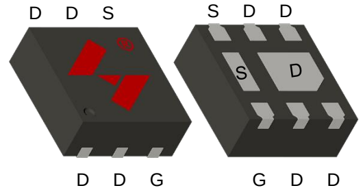
DFN6L(0202)
