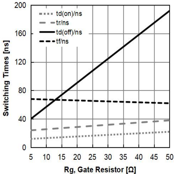
Figure 15: Typical Switching Times vs. Gate Resistor ( T_J=25^\circ\text{C} , V_{CE}=400V , V_{GE}=15/0V , I_C=20A )
