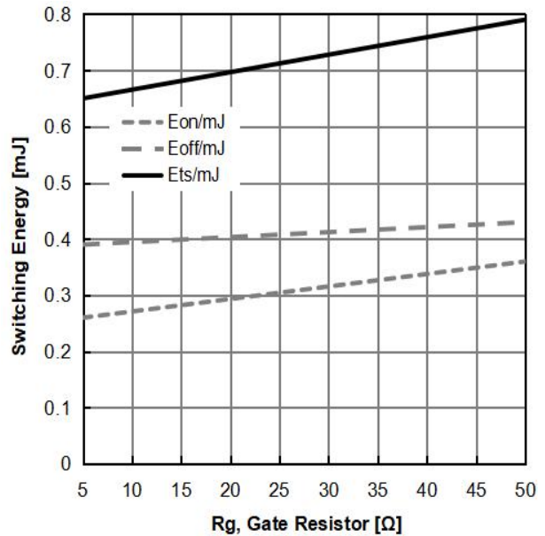
Figure 16: Typical Switching Energy vs. Gate Resistor ( T_J=25^\circ\text{C} , V_{CE}=400V , V_{GE}=15/0V , I_C=20A )
