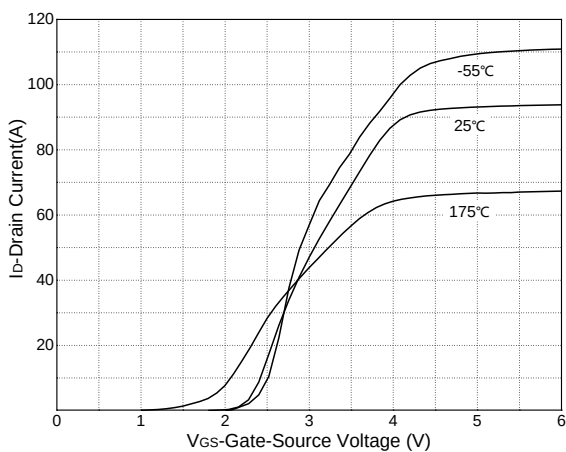
Figure 11: Transfer Characteristics
