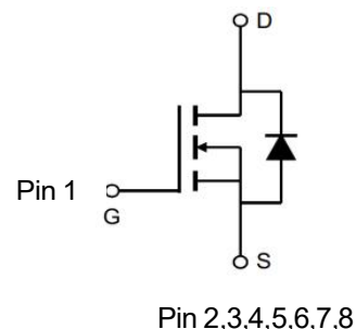
Single N-Channel MOSFET
