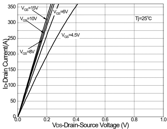
Figure 5: Output Characteristics
