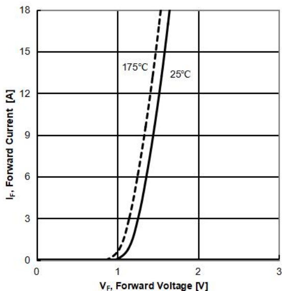
Figure 21: Typical Diode Forward Current vs. Forward Voltage
