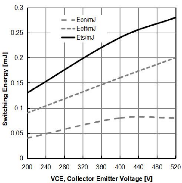
Figure 16: Typical Switching Energy vs. VCE ( T_J=25^{\circ}\text{C} , V_{GE}=15\text{V} , I_C=6\text{A} , R_g=5\Omega )
