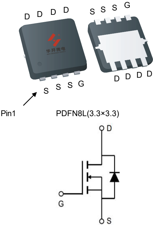
Single N-Channel MOSFET
