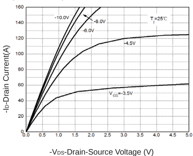
Figure 5: Output Characteristics
