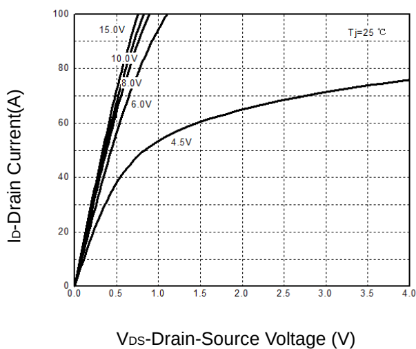
Figure 5: Output Characteristics
