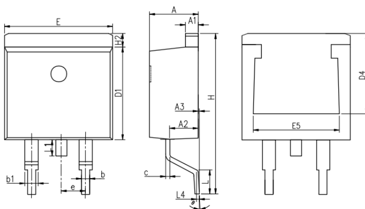
COMMON DIMENSIONS
