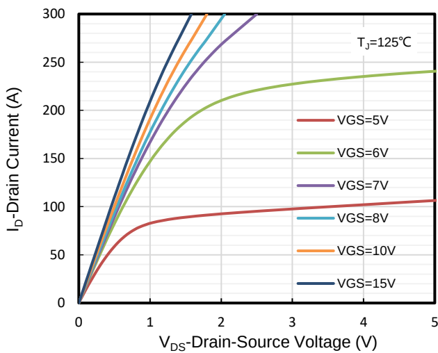
Figure 15: Output Characteristics ( 125^\circ C )
