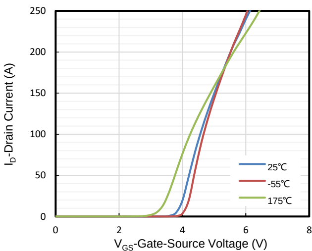
Figure 11: Transfer Characteristics
