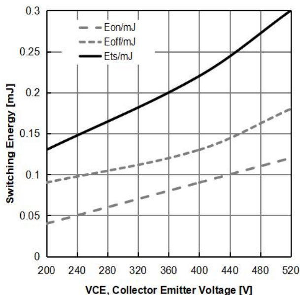
Figure 16: Typical Switching Energy vs. VCE ( T_J=25^{\circ}\text{C} , V_{GE}=15\text{V} , I_C=7\text{A} )
