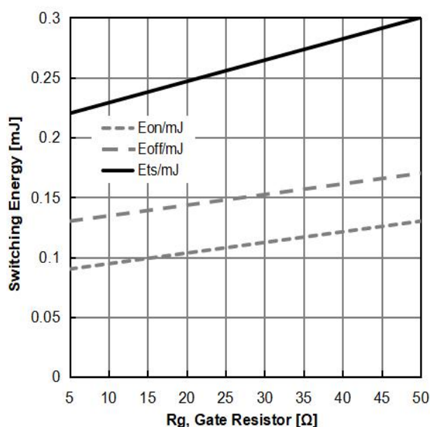
Figure 10: Typical Switching Energy vs. Gate Resistor ( T_J=25^\circ\text{C} , V_{CE}=400\text{V} , V_{GE}=15\text{V} , I_C=7\text{A} )
