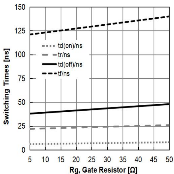
Figure 9: Typical Switching Times vs. Gate Resistor ( T_J=25^\circ\text{C} , V_{CE}=400\text{V} , V_{GE}=15\text{V} , I_C=7\text{A} )
