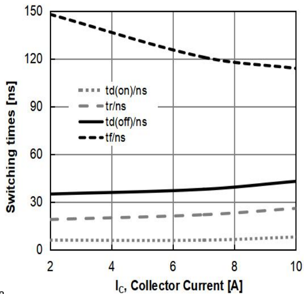
Figure 13: Typical Switching Times vs. Collector Current ( T_J=25^{\circ}C , V_{CE}=400V , V_{GE}=15V )
