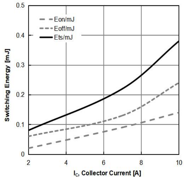
Figure 14: Typical Switching Energy vs. Collector Current ( T_J=25^{\circ}C , V_{CE}=400V , V_{GE}=15V )
