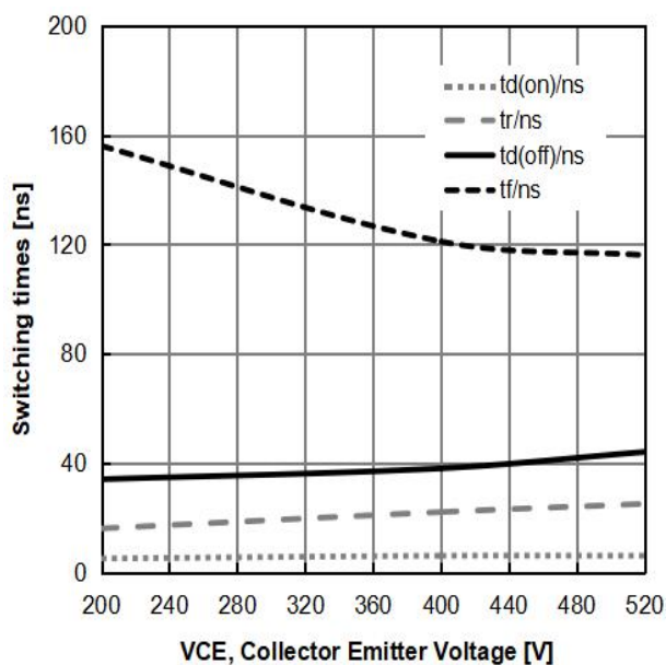
Figure 15: Typical Switching Times vs. VCE ( T_J=25^{\circ}\text{C} , V_{GE}=15\text{V} , I_C=7\text{A} )
