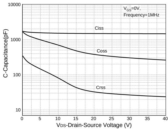
Figure 9: Capacitance Characteristics
